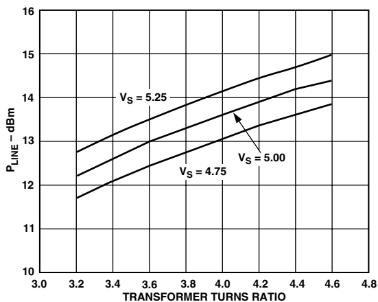
TPC 19. Line Power vs. Turns Ratio; MTPR = -65 dBc, f = 43 kHz
