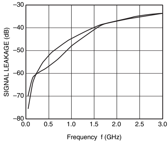
SIGNAL LEAKAGE vs. FREQUENCY (INx-OUT, all states)
