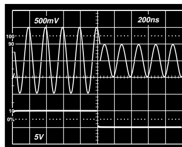
Figure 38. Channel Switching Characteristic for the 3:1 Mux
