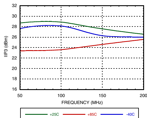
Figure 48. IP3 vs. IF Frequency at RF=2400 MHz, VGATE=5V
