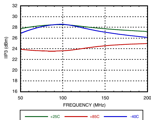
Figure 46. IIP3 vs. IF Frequency at RF=1900 MHz, VGATE=5V
