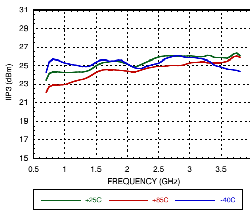
Figure 34. High Side LO Input IP3 vs. Frequency at VGATE=4.8V[2]
