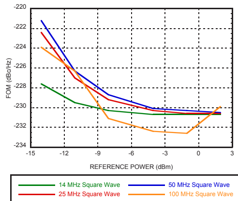
Figure 59. Reference Input Sensitivity, Square Wave, 50 Ω [3]
