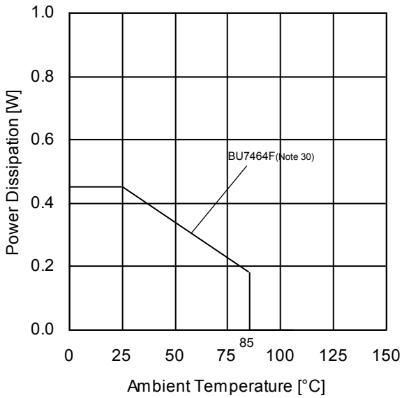
(g) BU7464F
