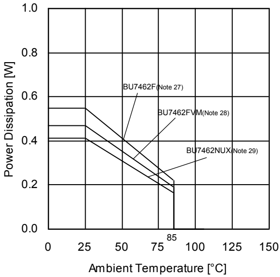
(e) BU7462xxx
