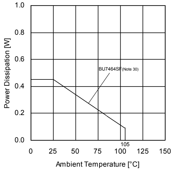
(h) BU7464SF
