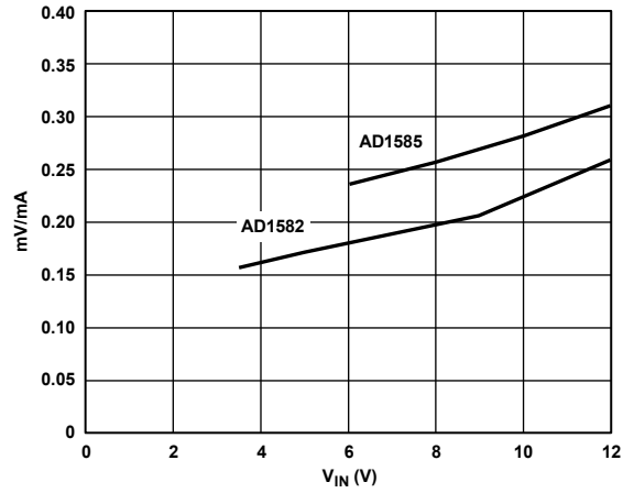
Figure 6. Load Regulation vs. V_{IN}
