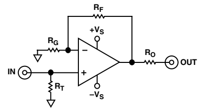
Noninverting Configuration
