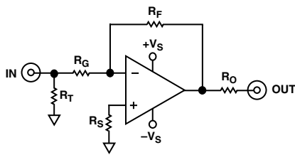
Inverting Configuration
