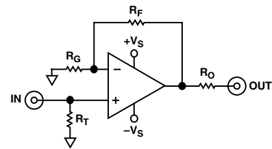
Noninverting Configuration
