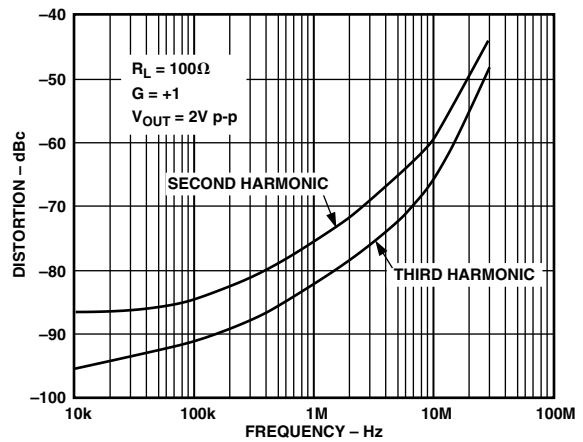
TPC 17. Distortion vs. Frequency, R_L = 100\Omega
