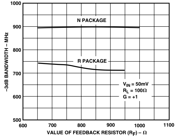
TPC 16. -3 dB Bandwidth vs. R_F , G = +1
