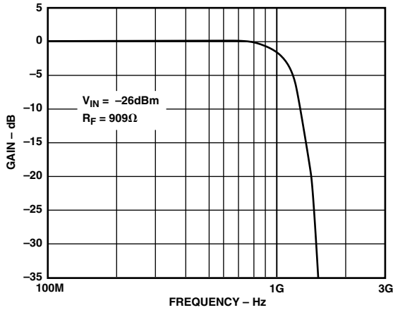
TPC 13. Frequency Response, G = +1
