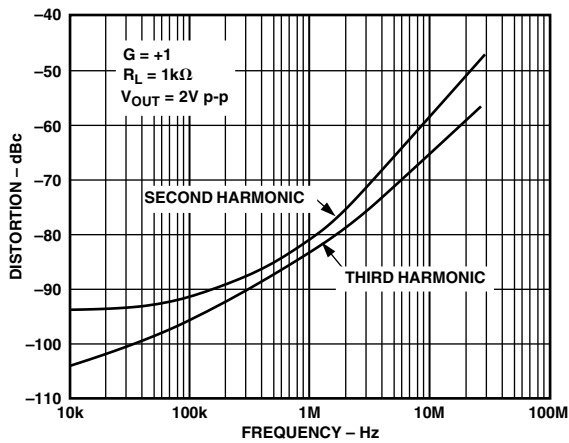
TPC 15. Distortion vs. Frequency, R_L = 1\text{k}\Omega
