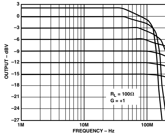
TPC 18. Large Signal Frequency Response, G = +1
