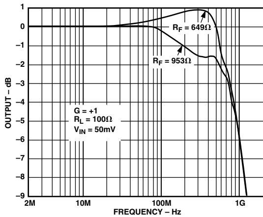
TPC 14. Flatness, R Package, G = +1 (for N Package Add 100\Omega to R_F )
