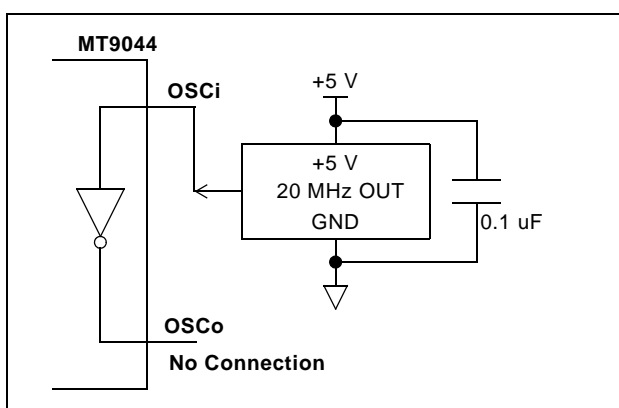
Figure 9 - Clock Oscillator Circuit
