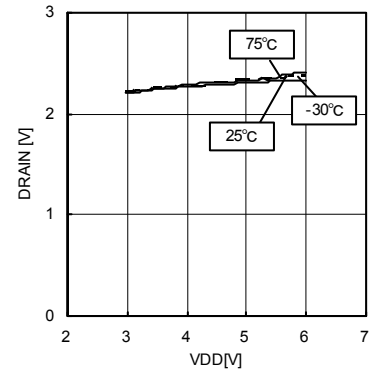
Fig.3 Drain Voltage (source 100µA)
