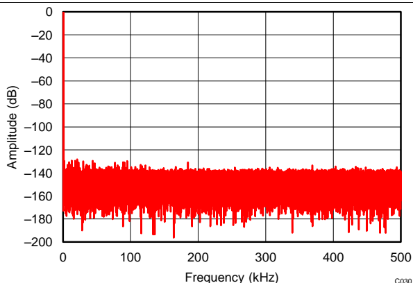
REF6241 driving REF pin of ADS8881, f_{IN} = 1\text{ kHz} , SNR = 99 dB, THD = -124.4 dB
