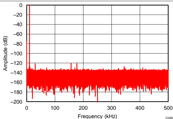
REF6225 driving REF pin of ADS8881, f_{IN} = 10\text{ kHz} , SNR = 94.0 dB, THD = -119.3 dB
