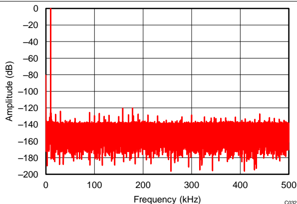
REF6241 driving REF pin of ADS8881, f_{IN} = 10\text{ kHz} , SNR = 97.2 dB, THD = -119.7 dB
