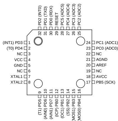
TQFP Top View
