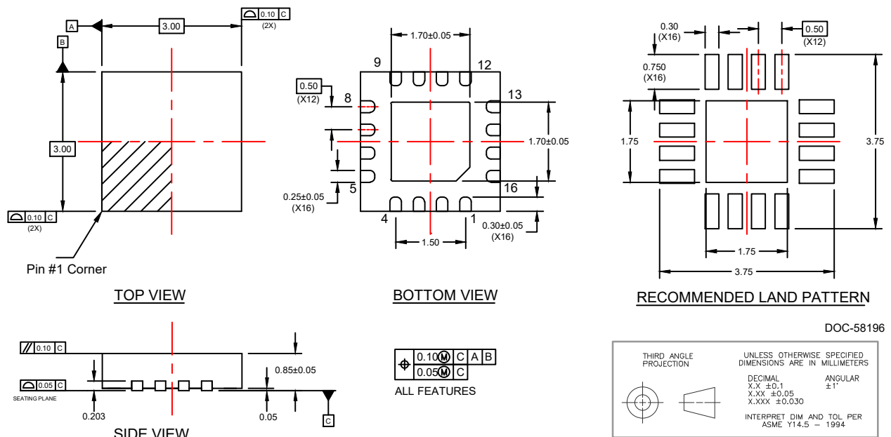
Figure 32. Package Drawing
