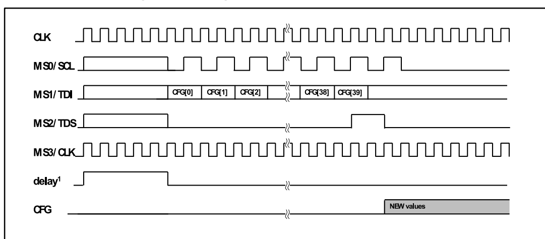
Figure 20: Timings to switch to soft mode after POR
