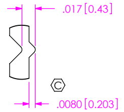
CRIMP DETAIL SCALE: 2X [TYP- ALL CRIMPS]
