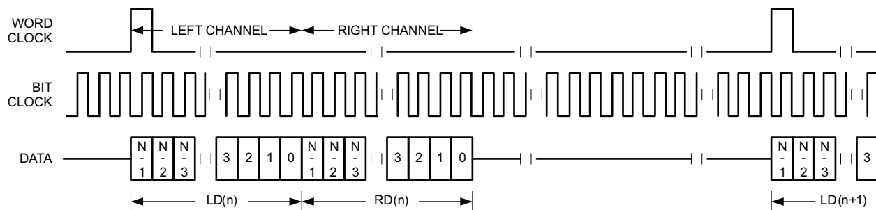
Figure 95. Timing Diagram for DSP Mode with Offset = 0 and Bit Clock Inverted
