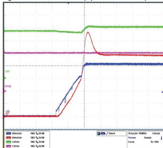
Figure 10. I_{VIN} , I_{LED} Startup ( I_{LED\_OUT} = 800mA )
