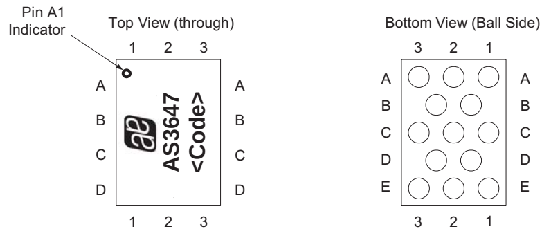
Figure 34. WL-CSP13 Marking AS3647
