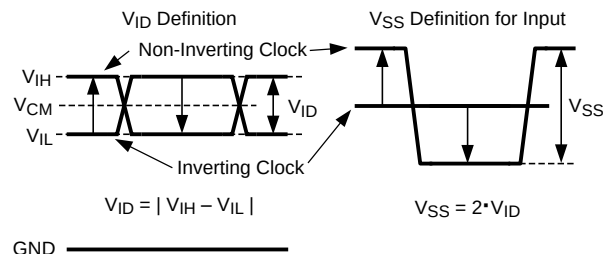
Figure 23. Two Different Definitions for Differential Input Signals
