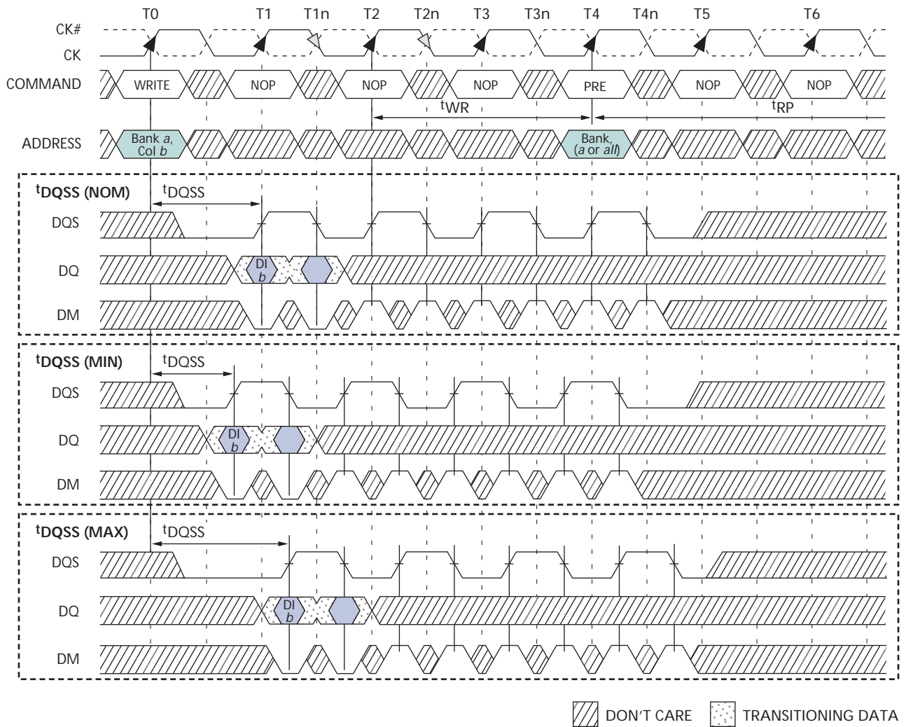
Figure 44: WRITE-to-PRECHARGE - Interrupting
