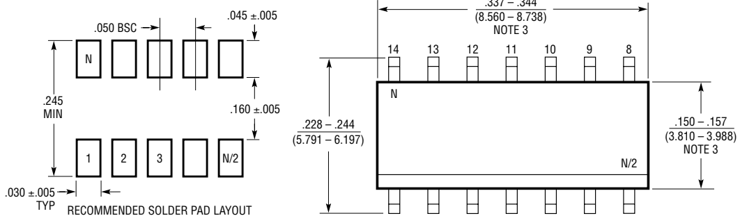
RECOMMENDED SOLDER PAD LAYOUT
