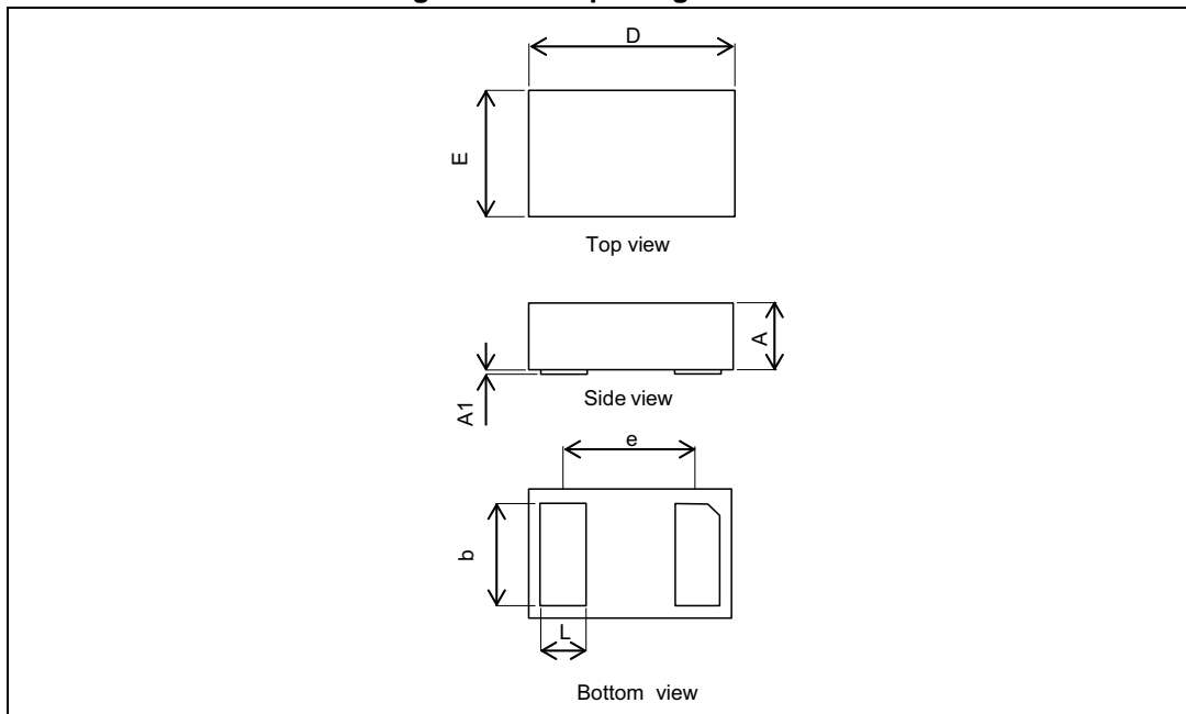
Figure 9. 1610 package outline
