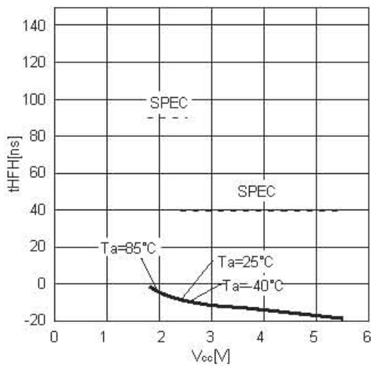
Figure 26. \overline{\text{HOLD}} setting hold time t_{HFH}
