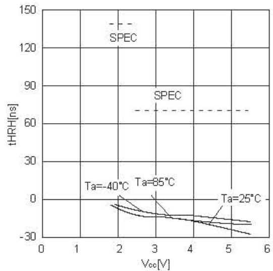
Figure 27. \overline{\text{HOLD}} release hold time t_{HRH}
