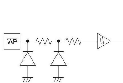
Figure 60. WP input equivalent circuit
