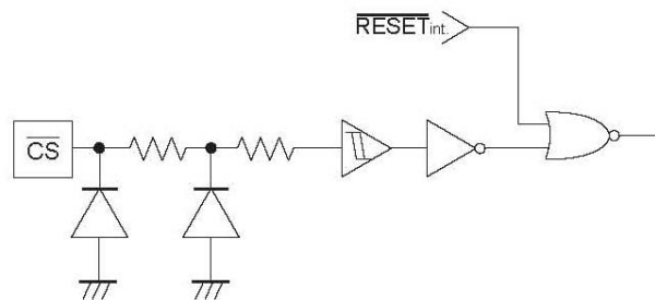
Figure 56. CS input equivalent circuit
