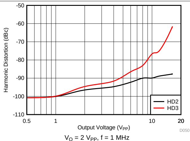
Figure 50. Harmonic Distortion vs Output Voltage
