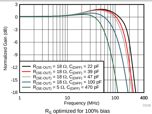
Figure 48. Frequency Response Across Capacitive Load
