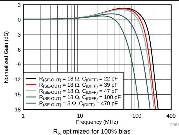
Figure 61. Frequency Response Across Capacitive Load
