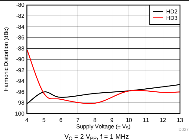
Figure 27. Harmonic Distortion vs Supply Voltage
