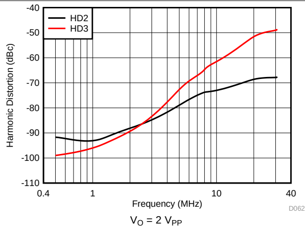
Figure 62. Harmonic Distortion vs Frequency
