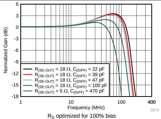
Figure 73. Frequency Response Across Capacitive Load
