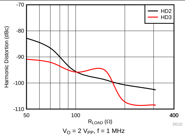
Figure 10. Harmonic Distortion vs Load Resistance
