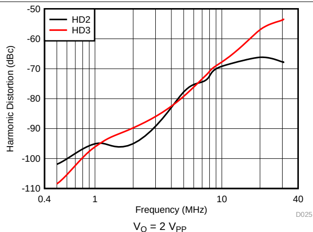
Figure 25. Harmonic Distortion vs Frequency
