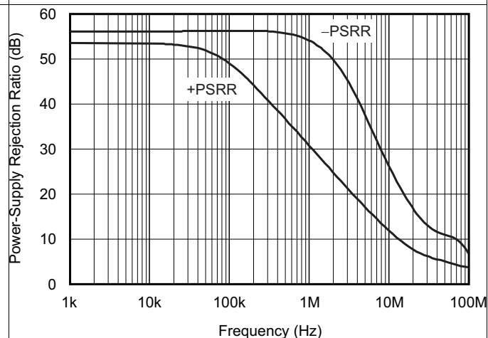
Figure 16. PSRR vs Frequency
