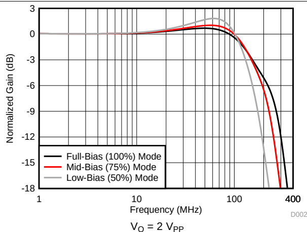
Figure 2. Small-Signal Frequency Response vs Bias Mode
