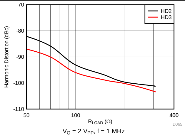
Figure 65. Harmonic Distortion vs Load Resistance
