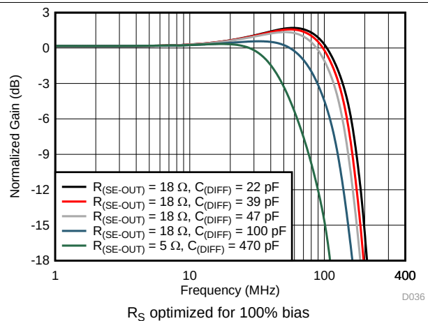
Figure 36. Frequency Response Across Capacitive Load
