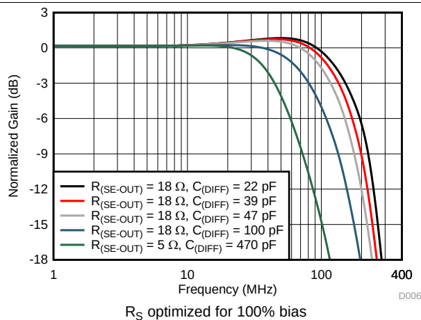
Figure 6. Frequency Response Across Capacitive Load
