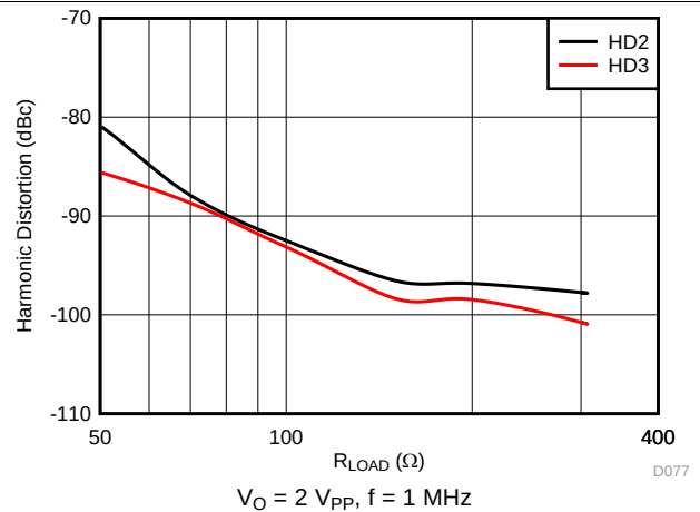
Figure 77. Harmonic Distortion vs Load Resistance
