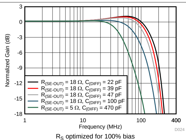
Figure 24. Frequency Response Across Capacitive Load
