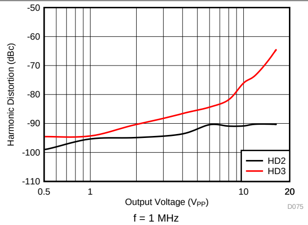
Figure 75. Harmonic Distortion vs Output Voltage
