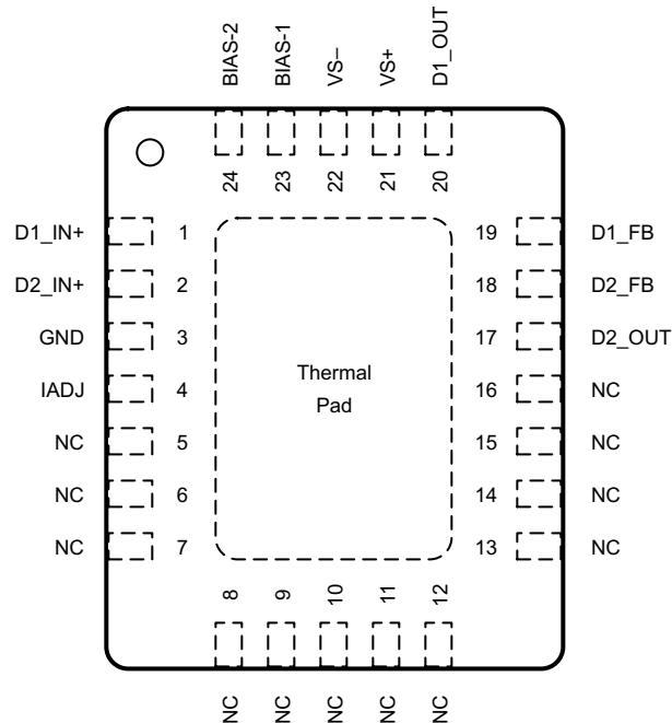
RHF Package 24-Pin VQFN With Exposed Thermal Pad Top View
