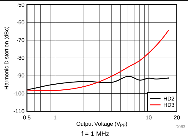
Figure 63. Harmonic Distortion vs Output Voltage
