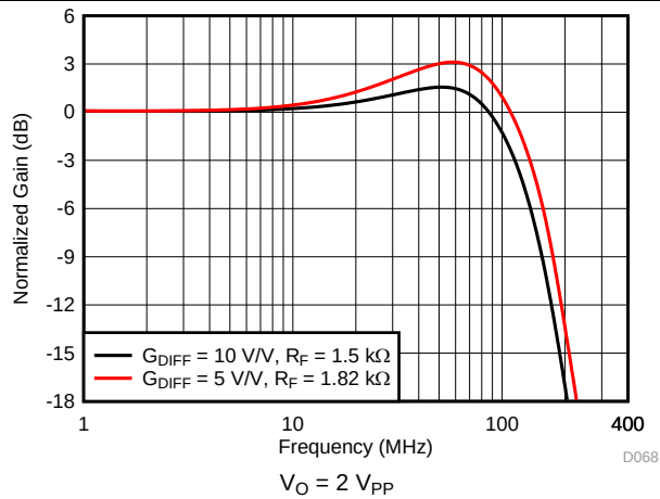
Figure 68. Small-Signal Frequency Response
