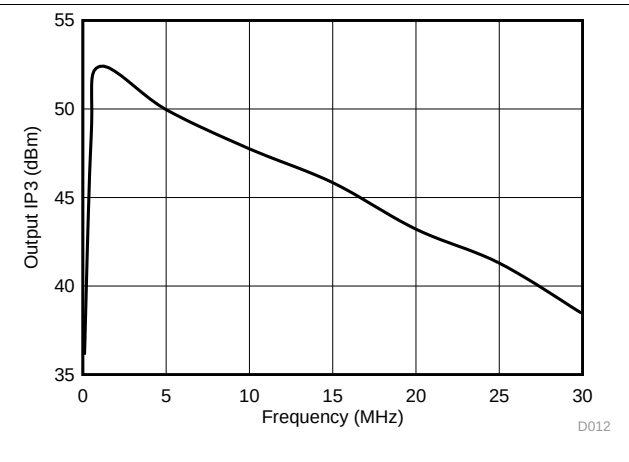
Figure 12. Two-Tone, Third-Order Intermodulation Intercept
