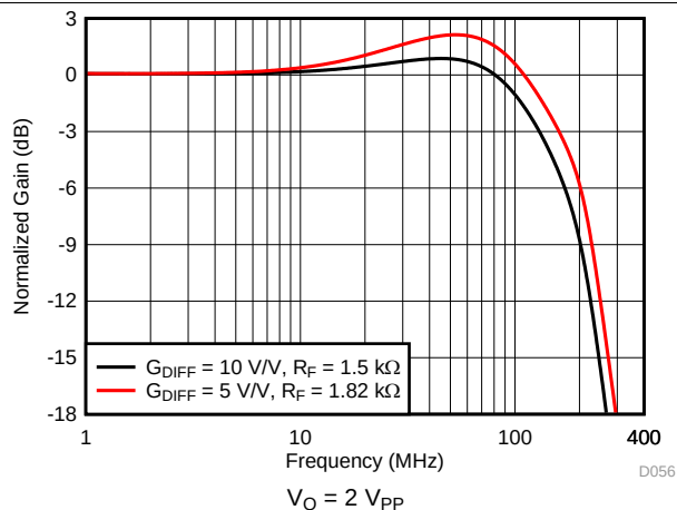
Figure 56. Small-Signal Frequency Response
