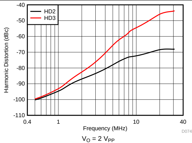
Figure 74. Harmonic Distortion vs Frequency
