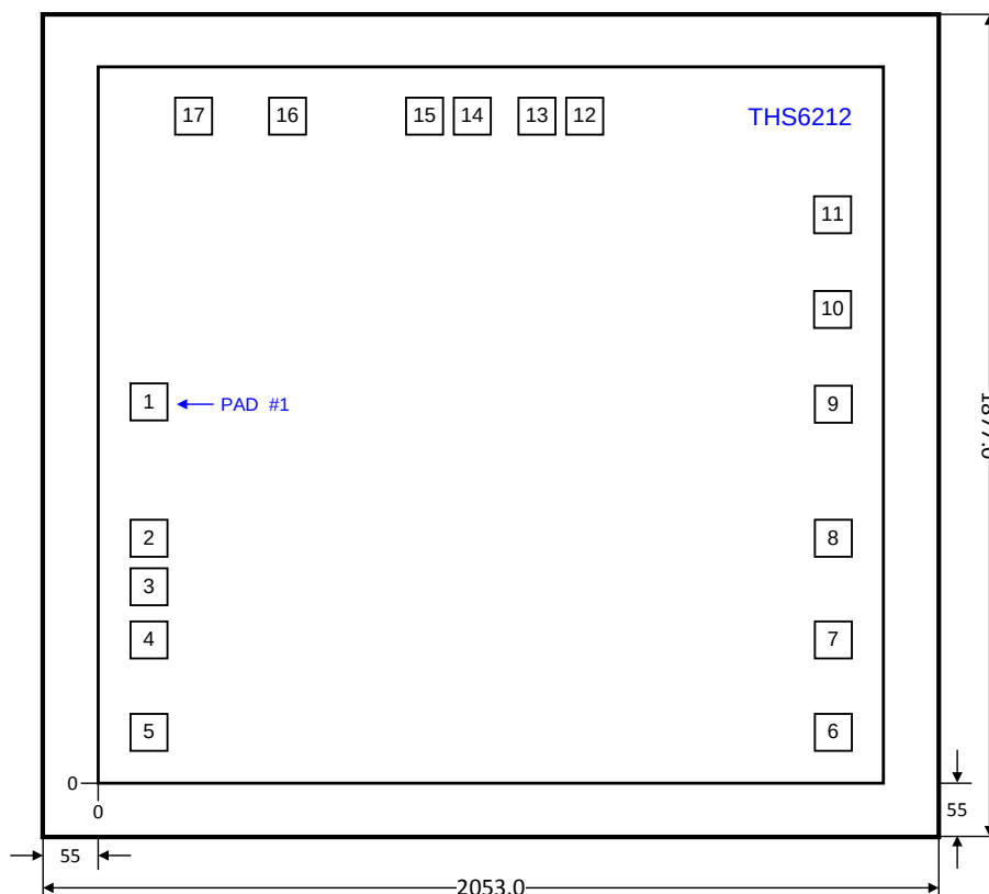
Figure 89. Die Dimensions
