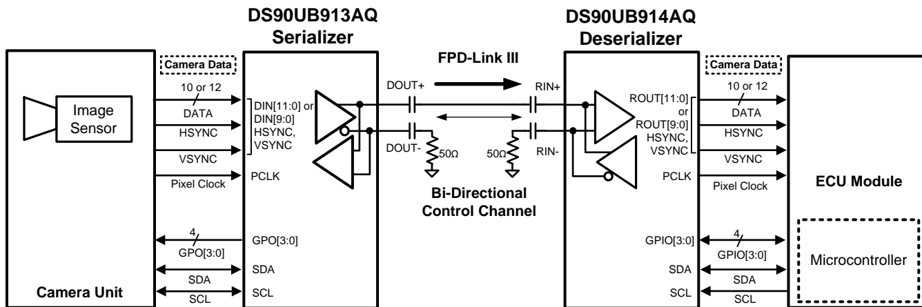
Figure 31. Coax Application Block Diagram
