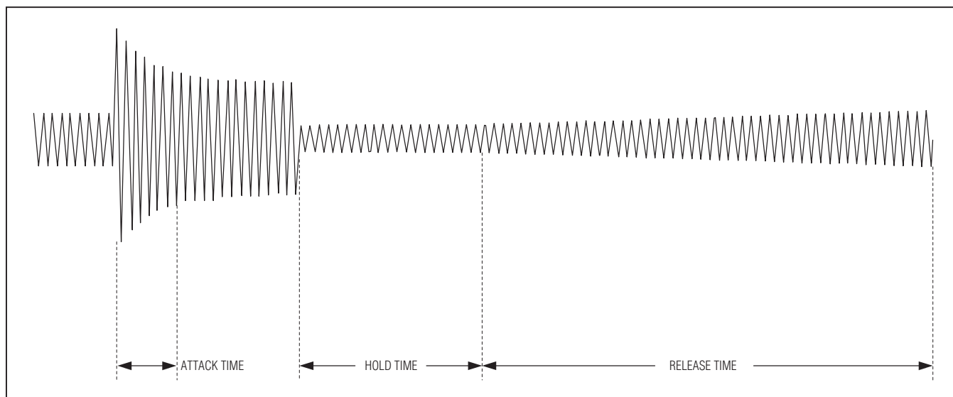
Figure 12. AGC Timing
