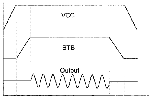
FIG 3. Standby ON/OFF Logic
