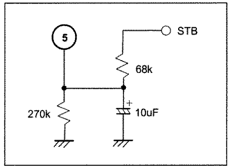
FIG 2. Standby Circuits
