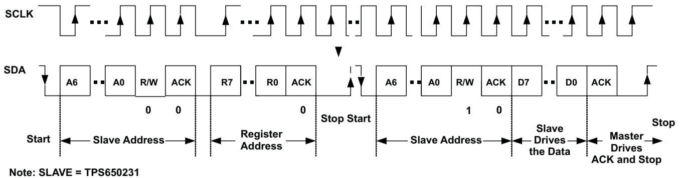
Figure 37. Serial I/F READ from TPS650231: Protocol B
