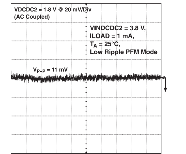
Figure 20. VDCDC2 Output Voltage Ripple
