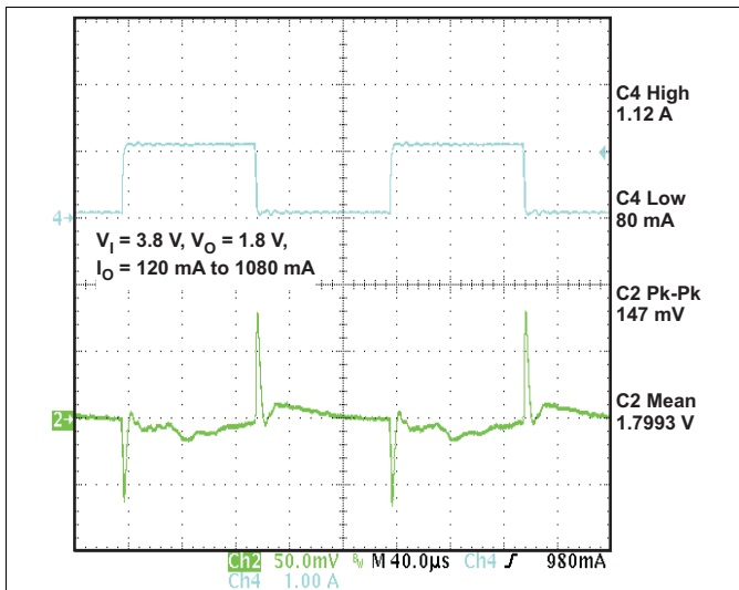
Figure 17. VDCDC2 Load Transient Response
