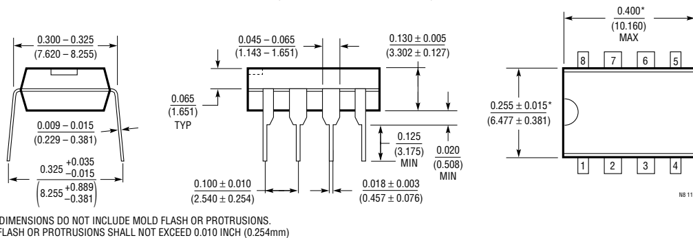
N8 Package 8-Lead PDIP (Narrow 0.300) (LTC DWG # 05-08-1510)
