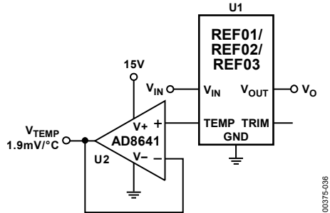
Figure 36. Temperature Monitoring
