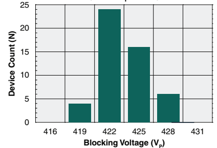
Typical Blocking Voltage Distribution (N=50, I F =0mA)
