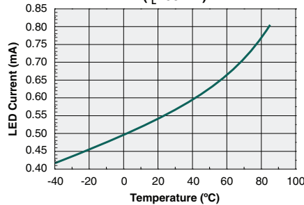
Typical I F for Switch Operation (I L =60mA)
