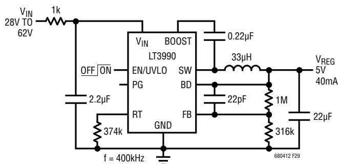
Figure 29. V_{\text{REG}} Powered from Cell Stack with High Efficiency
