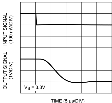
Figure 15. Settling Time (Falling Edge) at V_S = 3.3\text{ V} LMP8601 and LMP8601-Q1
