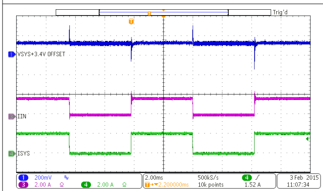
Figure 9-4. Charge Enable
