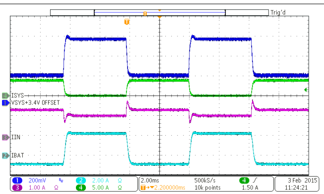
Figure 9-5. Charge Disable
