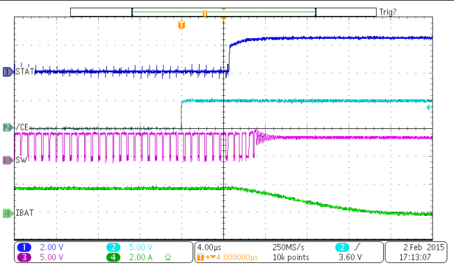
Figure 9-5. Charge Disable
