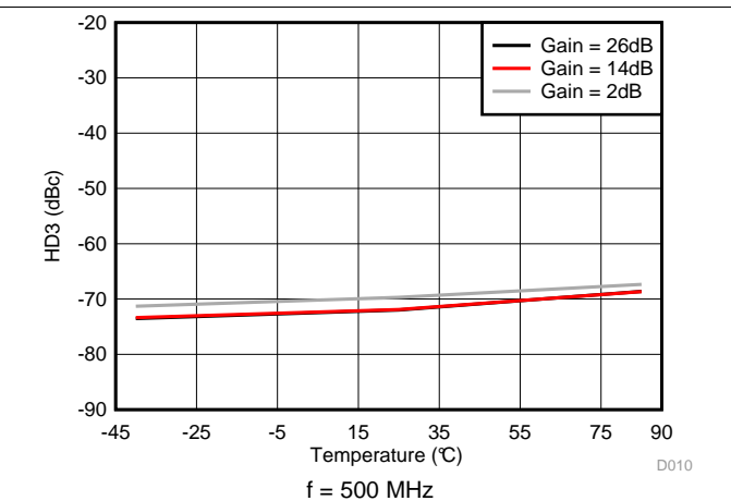
Figure 18. Third-Order Harmonic Distortion vs Temperature
