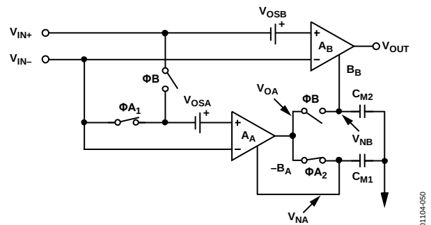
Figure 50. Auto-Zero Phase of the Amplifier
