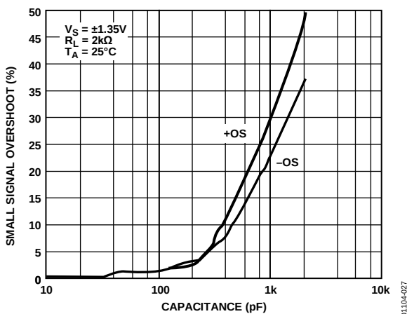
Figure 27. Small Signal Overshoot vs. Load Capacitance
