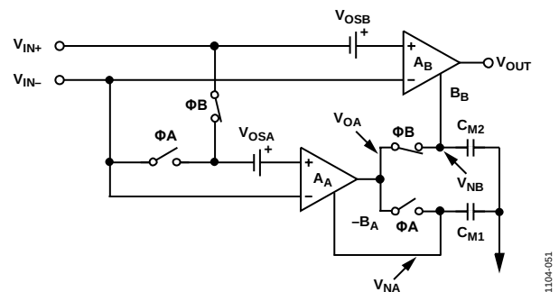
Figure 51. Output Phase of the Amplifier
