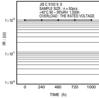
Fig.27 Insulation resistance
