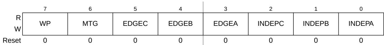
Figure 11-4. PMF Configure 0 Register (PMFCFG0)
