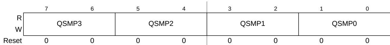
Figure 11-11. PMF Fault Qualifying Samples Register (PMFQSMP)
