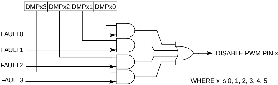
Figure 11-15. Fault Decoder
