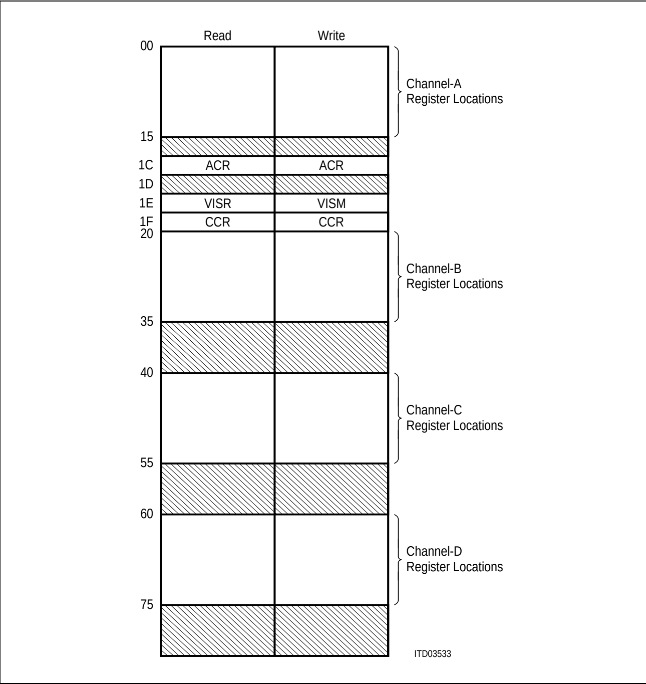
Figure 21 IDEC Register Map for Non-Multiplexed Address Bus
