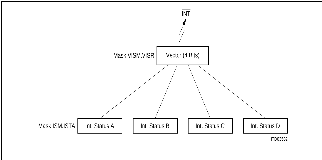
Figure 17 Interrupt Structure of the IDEC
