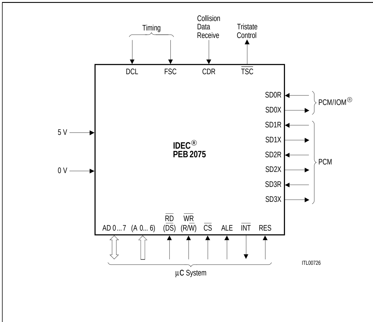
Logic Symbol
