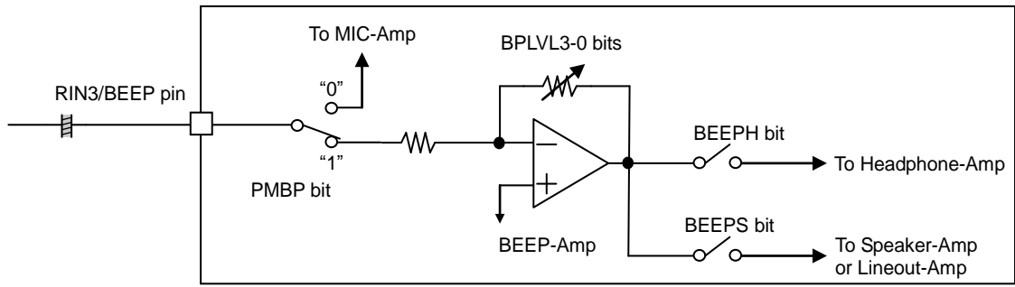
Figure 47. Block Diagram of BEEP pin
