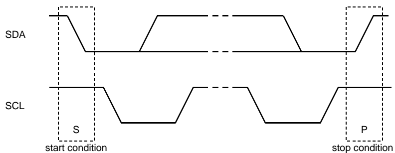
Figure 61. Start Condition and Stop Condition
