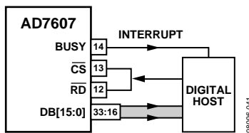
Figure 41. Interface Diagram—One AD7607 Using the Parallel Bus, with \overline{\text{CS}} and \overline{\text{RD}} Shorted Together
