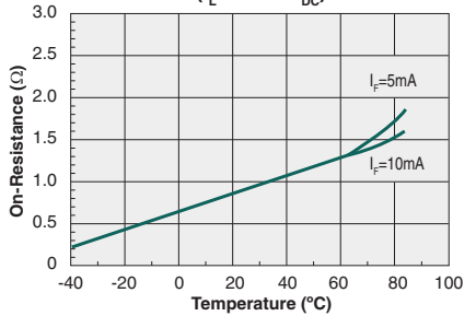
Typical On-Resistance vs. Temperature DC-Only Configuration ( I_L=350\text{mA}_{DC} )
