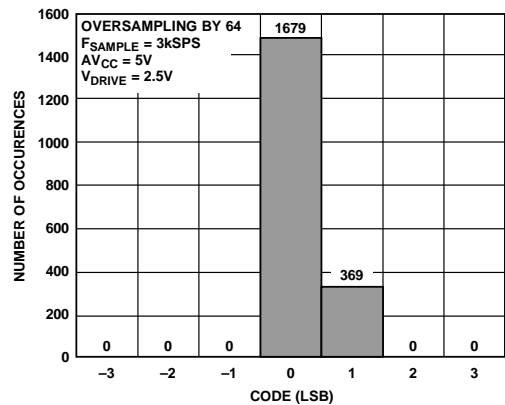
Figure 55. Histogram of Codes—OS \times 64 (Two Codes)
