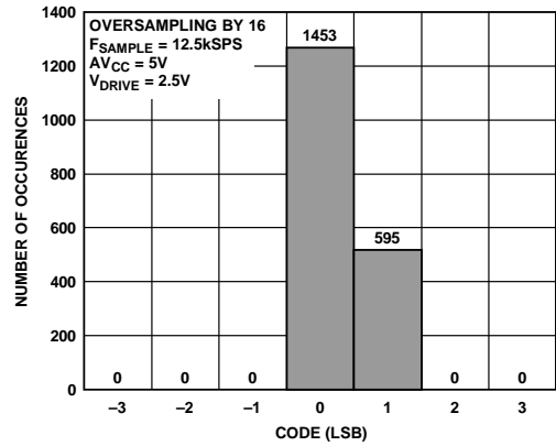
Figure 53. Histogram of Codes—OS \times 16 (Two Codes)
