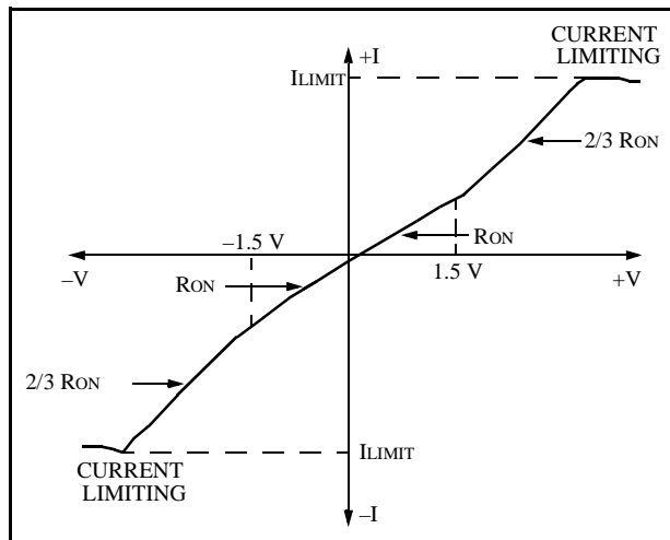
Figure 4 - Switches 3, 7, 9, and 10
