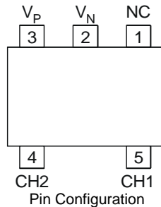
Pin Configuration
