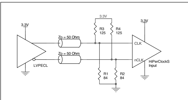
FIGURE 2C. HiPerClockS PCLK/nPCLK INPUT DRIVEN BY A 3.3V LVPECL DRIVER
