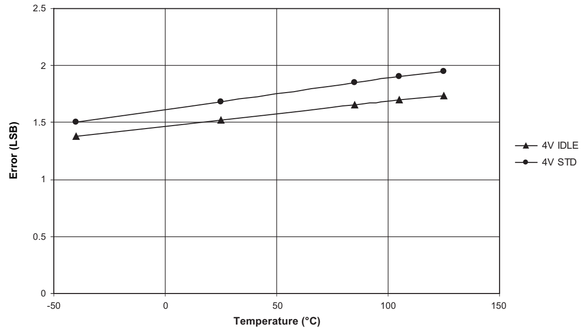
Figure 28-28. Analog to Digital Converter OFFSET versus V CC
