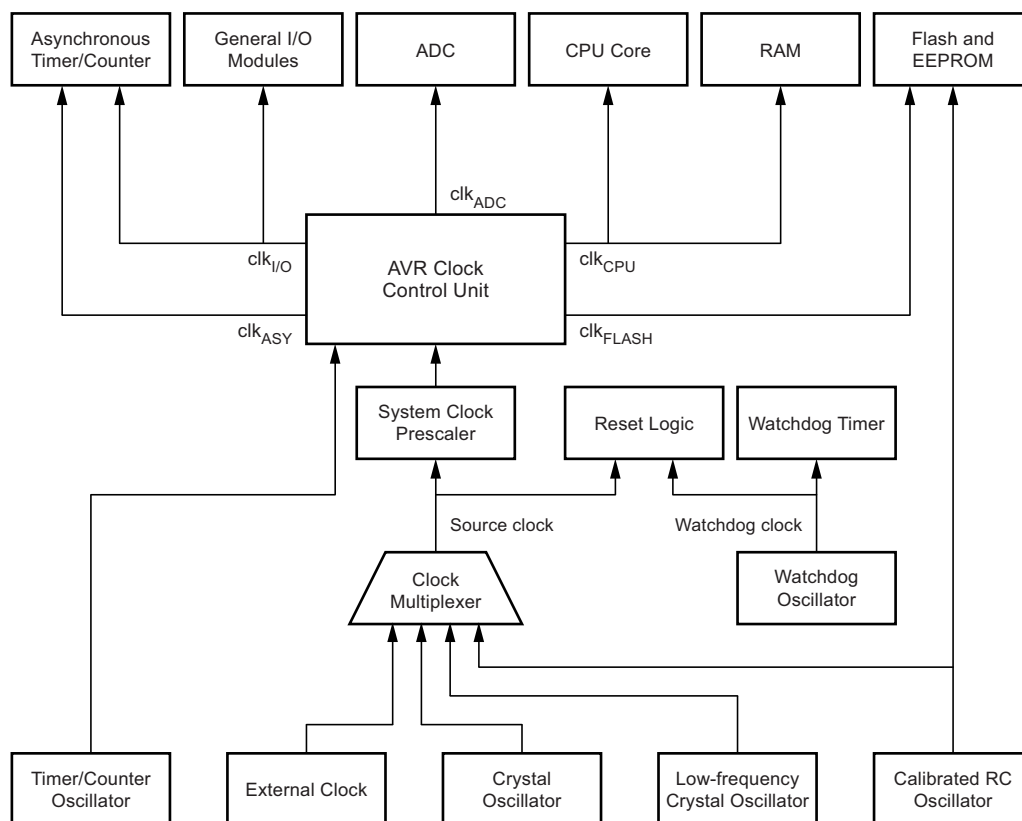
Figure 6-1. Clock Distribution
