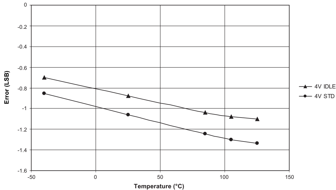
Figure 28-27. Analog to Digital Converter GAIN versus V CC
