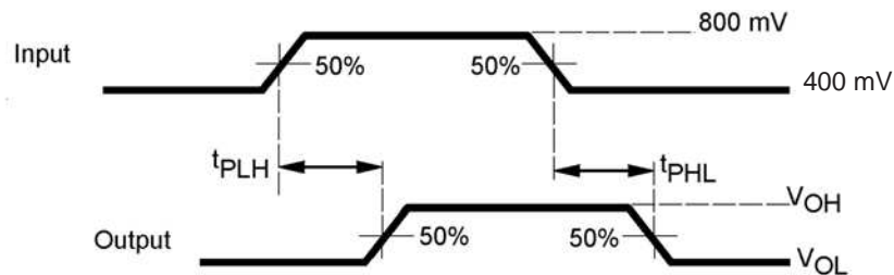
Figure 10. Propagation Delay
