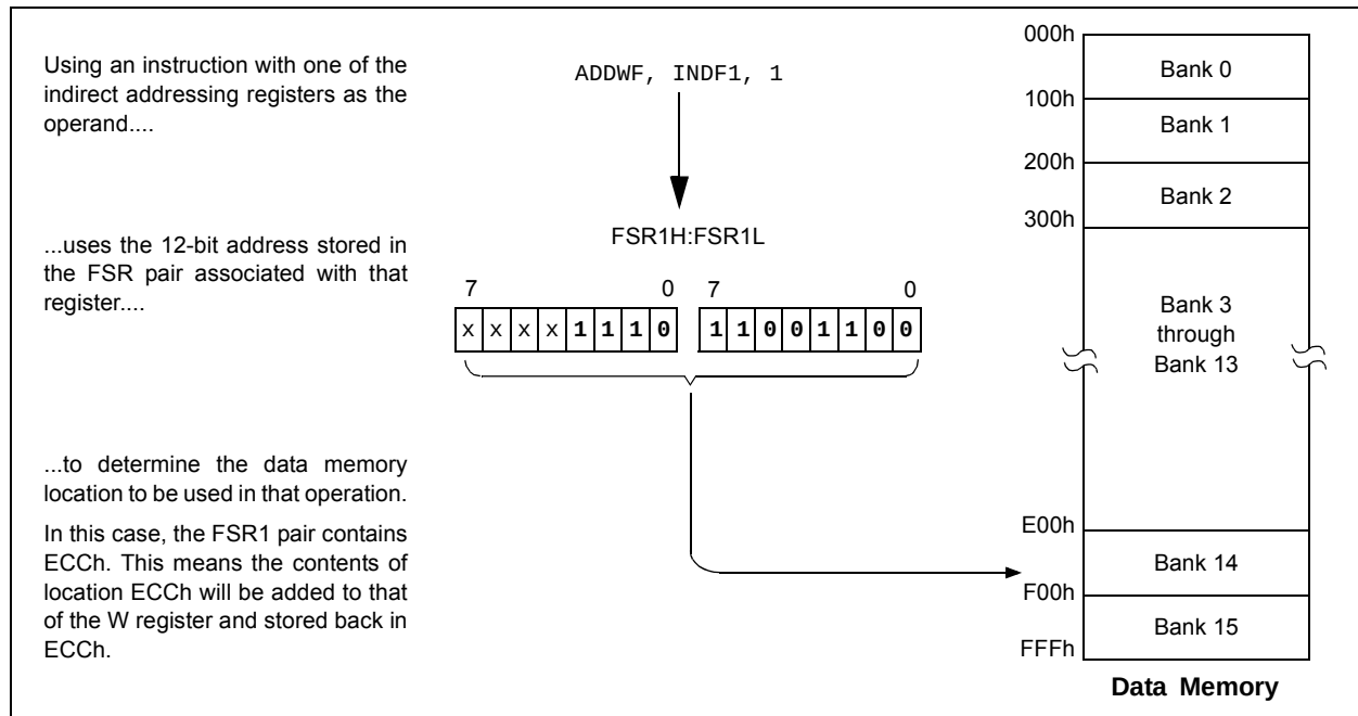
FIGURE 6-7: INDIRECT ADDRESSING
