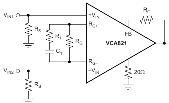
Figure 83. Differential Equalizer
